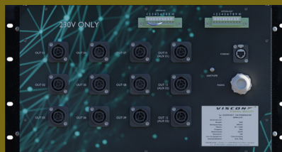
EPPM 32 / 32+ Rear View
